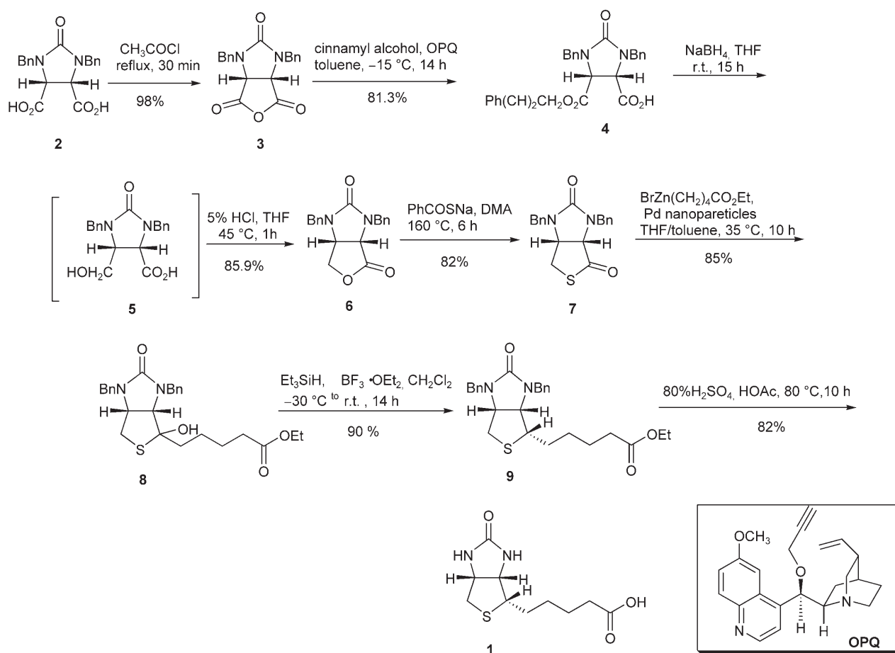
Scheme 1. The synthetic route to (+)-biotin ( 1 ).
