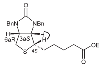
Figure 2. 2D NOESY interactions of compound 9 .
