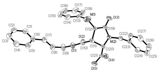
Figure 1. The structure and absolute configuration of 4 .
